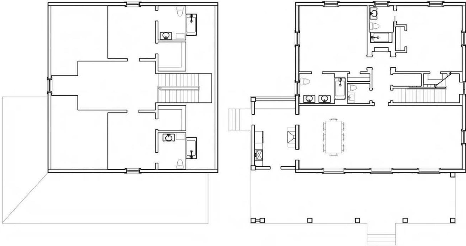
CLUB VILLA Xa 1ST & 2ND FLOOR PLAN
